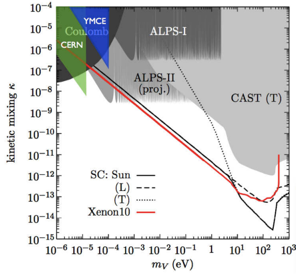
Figure 4: Updated from [13]. The filled in region labeled YMCE denotes the exclusion set by our experiment. This result and the limit from the CERN experiment (Ref. [7]) are the first microwave cavity LSW experiments to surpass the Coulomb limit; the region labeled ALPS-II [5] is the projected sensitivity of future optical LSW experiments.
