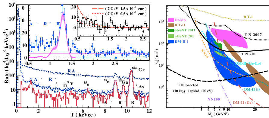
Figure 3: (left) Measured energy spectra, showing the raw data and those with \text{AC}^- \otimes \text{CR}^- (\otimes \text{B}') selections. The large inset shows the (\epsilon_{\text{BS}}, \lambda_{\text{BS}}) -corrected \text{AC}^- \otimes \text{CR}^- \otimes \text{B} , with a flat background and L-shell X-ray peaks overlaid. The small inset depicts the residual spectrum superimposed with that due to an allowed (excluded) cross-section at m_\chi = 7 GeV. (right) Exclusion plot of spin-independent \chi\text{N} coupling at 90% confidence level, superimposed with the results from other benchmark experiments.
