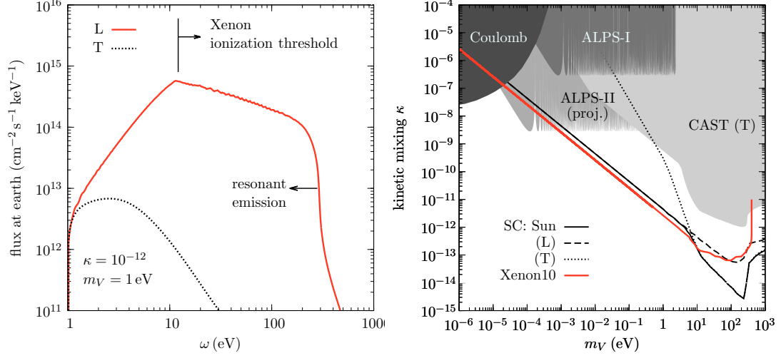
Figure 1: Left : Energy differential solar dark photon flux at Earth for \kappa = 10^{-12} and m_V = 1 eV. The solid/dotted line shows the longitudinal(L)/transverse(T) contribution. Right : Constraints on \kappa as a function of m_V . The black solid/dashed/dotted curves show the total/longitudinal/transverse energy loss limit of the Sun by requiring that the dark photon luminosity does not exceed 10% of the standard solar luminosity [7]. The red line shows the constraint derived from the XENON10 data. Previous and future (“proj.”) experimental bounds/sensitivities are shown by the shaded regions. From light to dark shading these are from the CAST experiment [8] considering the contributions from only the transverse modes [2], from the ALPS collaboration [9], and from tests of the inverse square law of the Coulomb interaction [10].
