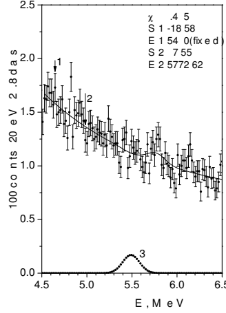
Figure 3: The fitted BGO spectrum in the (4.5 – 6.5) MeV range. Curve 3 is the detector response function for E_0 = 5.49 MeV and \sigma = 0.093 MeV.
