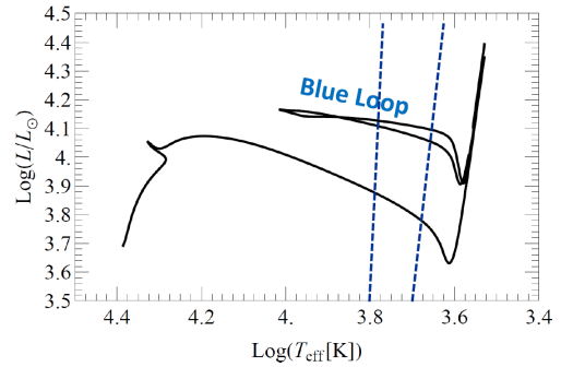
Figure 1: Evolution in the HR diagram of a 9.5 M_{\odot} star. The region between the two dashed lines is the instability strip, where the Cepheid variables are found.
