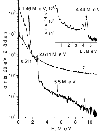
Figure 2: The energy spectrum of the BGO detector measured (1) in anticoincidence and (2) in coincidence with the active shielding signal. The location of the expected 5.5 MeV axion peak is denoted by an arrow. In inset the spectrum measured with Pu-Be neutron source is shown.
