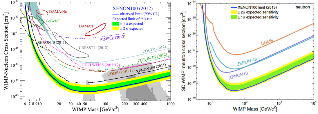
Figure 1: WIMP-nucleon cross section exclusion limits from 225 live days run of XENON100. (Left) Spin-independent. (Right) Spin-dependent (neutron coupling). Figures from [4] and [2], respectively.
