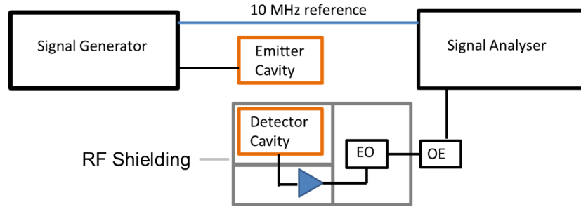
Figure 2: Schema of the measurement setup. The amount of shielding around the detector cavity will be increased according to the requirements of the measurements. Also the optical conversions will not be used in the first measurements but will be developed and implemented when required.
