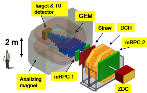
Figure 4: BM@N detector.
