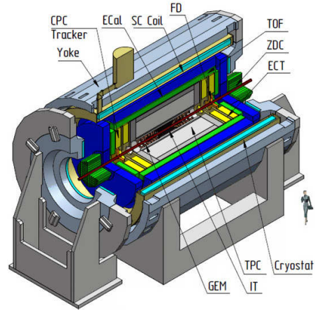
Figure 2: MPD detector.
