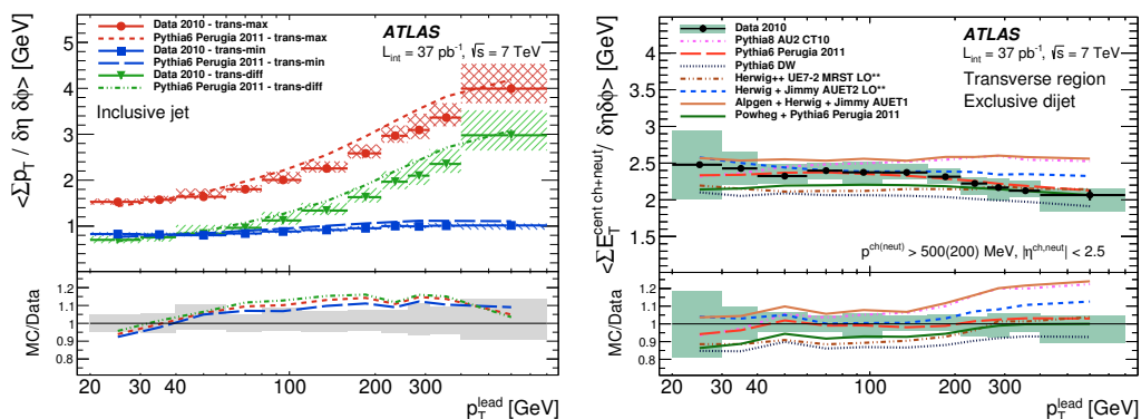
Figure 1: Comparison of profiles of charged-particle \sum p_T left (neutral and charged \sum E_T right) as a function of p_T^{lead} in transverse regions for ATLAS measurements and MC predictions.
