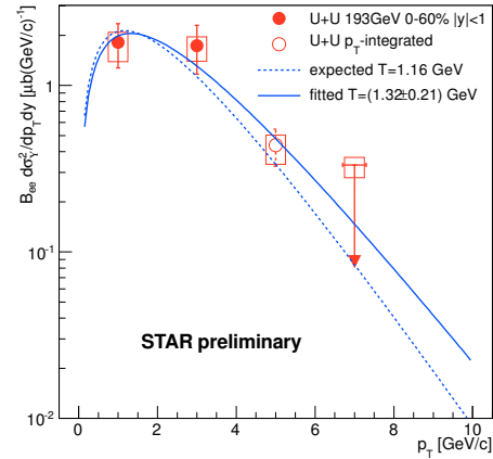
Figure 2: \Upsilon p_T -spectrum in \sqrt{s_{NN}}=193 GeV U+U collisions of 0–60% centrality at mid-rapidity. The fit (solid line) to the data is compared to the expected slope (dashed).
