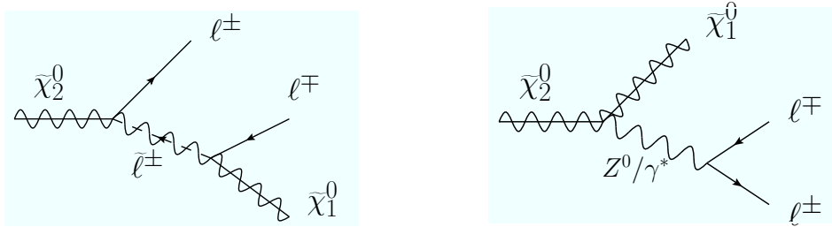
Figure 1: Diagrams of the possible decay modes of the second neutralino resulting in an edge in the dilepton invariant mass spectrum.
