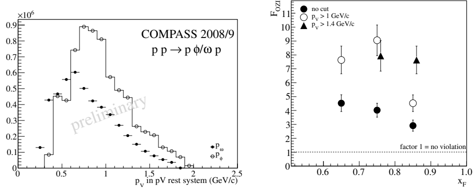
Figure 1: Left: The vector meson momentum p_V in the rest frame of the pV system, where V refers to \phi (white dots) or \omega (black dots). The \phi histogram has been scaled by a factor of 100. Right: OZI violation factor F_{\text{OZI}} as a function of x_F for different p_V cuts.
