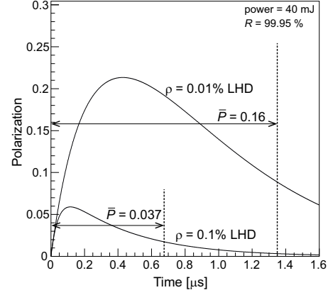
Figure 2: Time population of the muon spin polarization.
