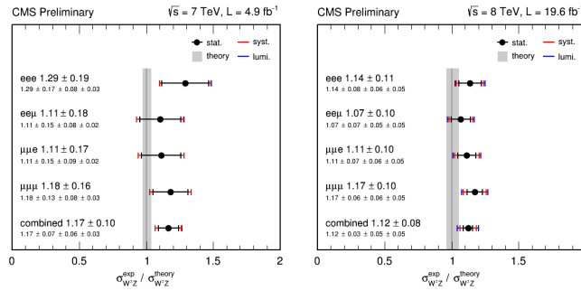
Figure 1: Ratio of measured inclusive cross-section to the theoretical prediction in the WZ \rightarrow l\nu l\ell channel at \sqrt{s} = 7 TeV(left) and \sqrt{s} = 8 TeV(right).
