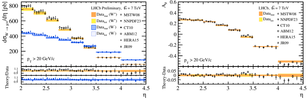
Figure 1: W^+ and W^- cross-sections (left) and lepton charge asymmetry (right) as a function of muon pseudorapidity [2]. The measurements, shown as coloured bands, are compared to NNLO predictions with different PDF sets. They are displaced horizontally for better visibility.
