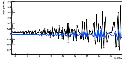
Figure 3: Ratio for neutrinos which have undergone propagation decoherence (blue) and neutrinos which have undergone graviton induced decoherence (black).
