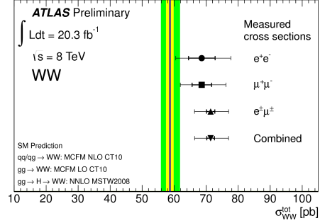
Figure 2: W^+W^- cross section [8].
