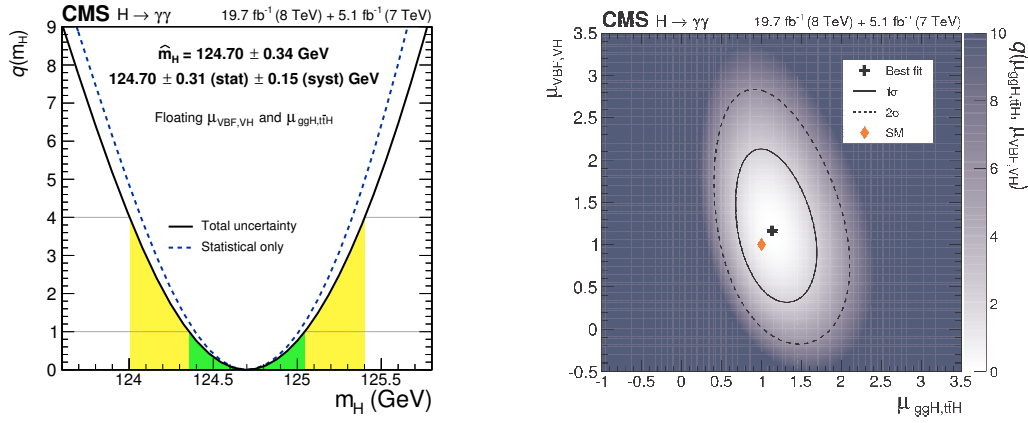
Figure 2: Left: likelihood scan as a function of the mass with \mu_{ggH,tH} and \mu_{VBF,VH} floated independently. Right: likelihood scan as a function of \mu_{ggH,tH} and \mu_{VBF,VH} ; the 1\sigma and 2\sigma uncertainty contours are shown, the cross indicates the best-fit values and the diamond represents the standard model expectation.
