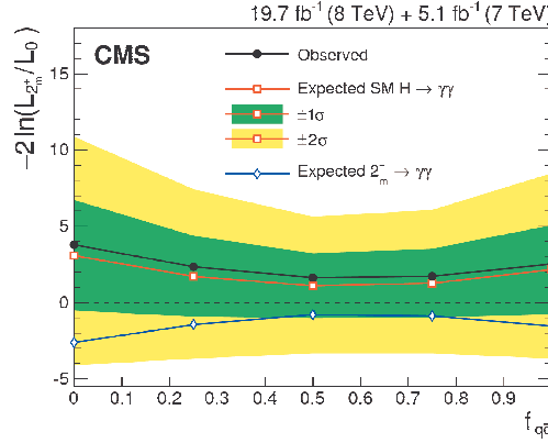
Figure 3: Test statistic for pseudo-experiments generated under the standard model 0^+ hypothesis (open squares) and the graviton-like 2_m^+ hypothesis (open diamonds), as a function of the fraction f_{q\bar{q}} of q\bar{q} production. The full dots correspond to the observed distribution in the data.
