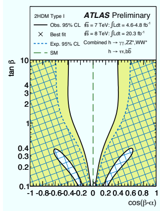
Figure 1: Regions of the (\cos(\beta - \alpha), \tan(\beta)) plane for a coupling configuration of 2HDMs excluded by fits to the measured rates of the Higgs boson production and decays. The cross marks the best fit value, the light shaded and hashed regions indicate the observed and expected 95% confidence level exclusions. [10]
