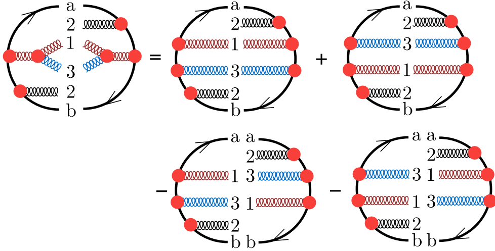
Figure 8. Identity for color dependence of splitting of gluon 1 in both the bra state and the ket state in the case \{c'\}_m \neq \{c\}_m . In the LC+ approximation, one keeps all four terms. In the LC approximation, we keep only the first two terms.
