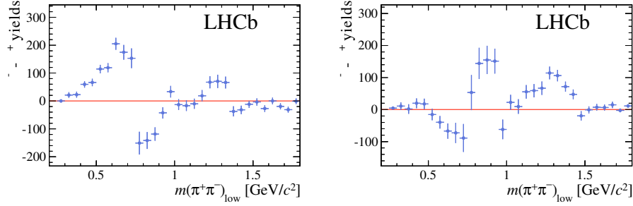
Figure 4: Difference of the B^- and B^+ signal yields as a function of the \pi^+\pi^- invariant mass in the B^\pm \rightarrow \pi^\pm\pi^+\pi^- decay. The yields have been background-subtracted and efficiency-corrected.
