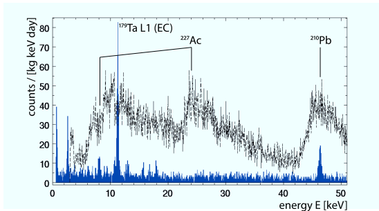
Figure 2: Background spectra for a commercial \text{CaWO}_4 crystal ( open black histogram ) and TUM40 ( filled blue histogram ). Prominent features are the beta decays of ^{227}\text{Ac} and ^{210}\text{Pb} , and the electron capture of cosmogenic ^{179}\text{Ta} [6, 11].
