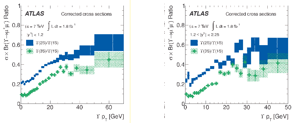
Figure 3: The relative production of prompt \Upsilon 2S to \Upsilon 1S and \Upsilon 3S to \Upsilon 1S with respect to the p_T of the \Upsilon in the central (left) and forward (right) regions.
