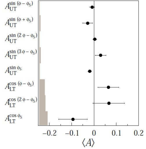
Figure 3: Target spin asymmetries on \mu p^{\uparrow\downarrow} \rightarrow \mu p \rho^0 measured at COMPASS [6, 7].
