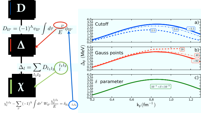
Figure 1: Left: Self-consistent procedure (Eqs. 7–9) for the solution of the gap equation according to Khodel’s prescription [6]. Right: Numerical analysis of Khodel’s procedure for the singlet channel in neutron matter: a) cutoff, b) Gaussian integration points and c) \delta dependence. This method is a very stable procedure if satisfactory values of n_{gauss} and \Lambda_k are employed.
