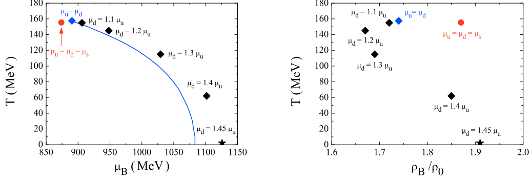
Figure 1: The influence of the isospin in the location of the CEP within the PNJL model: the full line is the first order phase transition line for zero isospin matter ( \mu_u = \mu_d , \mu_s = 0 ). The chemical potential for the strange quark is always taken equal to zero, except the for the red point ( \mu_u = \mu_d = \mu_s ) which is given for reference. When \mu_d > 1.45\mu_u the CEP doesn't exist anymore.
