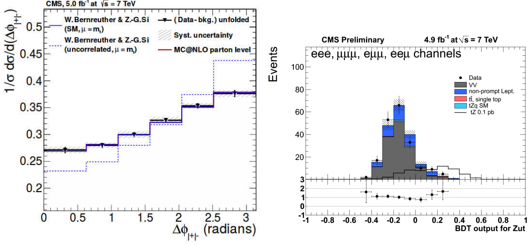
Figure 2: Left, \Delta\phi(\ell\ell) differential cross section in t\bar{t} events. Right : BDT distribution after the tZ selection.
