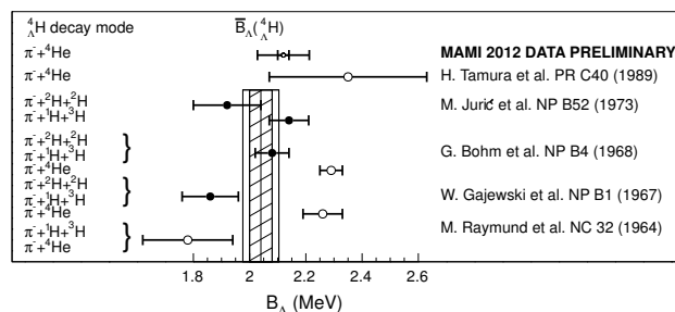
Figure 4: Measurements of the binding energy of {}^4_{\Lambda}\text{H} determined from different pionic decays. Details are discussed in the text.
