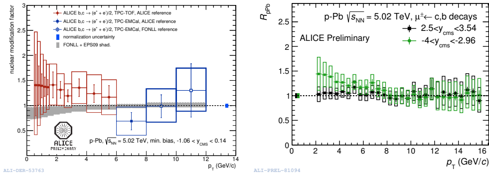
Figure 1: R_{\text{pPb}} of heavy-flavour decay electrons at mid-rapidity and heavy-flavour decay muons at forward (p-going direction) and backward (Pb-going direction) rapidities in minimum-bias p-Pb collisions, as a function of p_{\text{T}} .
