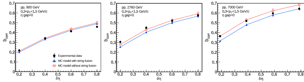
Figure 1: Correlation coefficient as a function of the pseudorapidity windows width ( \delta\eta ) at midrapidity ( \eta_{\text{gap}} = 0 ). Lines – the results of calculation in the model with and without string fusion, points – the experimental data [2].
