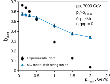
Figure 2: Correlation coefficient as a function of the lower transverse momentum bound. Line – the result of calculation in Monte Carlo model with string fusion, points – the experimental data [3].
