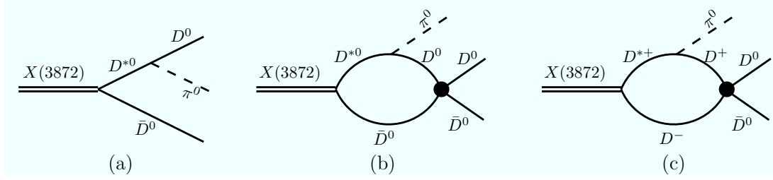
Figure 1: Feynman diagrams for the decay X(3872) \rightarrow D^0 \bar{D}^0 \pi^0 . The charge conjugate channel is not shown but included in the calculations.
