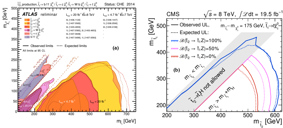
Figure 7: (a) Exclusion limits for top squark pair production from ATLAS [32, 33, 34, 35] shown in the m_{\tilde{t}_1}-m_{\tilde{\chi}_1^0} plane. (b) Exclusion limits for \tilde{t}_2 -pair production for different branching fractions of \tilde{t}_2 \rightarrow Z(H)\tilde{t}_1 [37].
