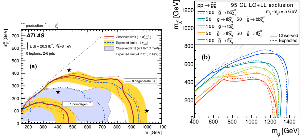
Figure 6: (a) Squark mass limits in the m_{\tilde{q}}-m_{\tilde{\chi}_1^0} plane [25], and (b) gluino mass limits in the m_{\tilde{g}}-m_{\tilde{\chi}_1^0} plane obtained for different gluino branching fraction models [27].
