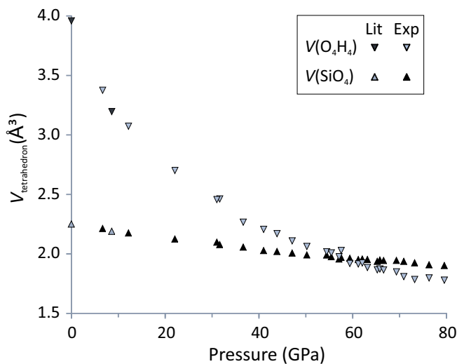
FIG. 4. Volume compression of the O_4H_4 and SiO_4 tetrahedra in henritermierite obtained from experiment and literature [8]. At about 55 GPa the large and highly compressible O_4H_4 tetrahedron is compressed to a similar volume as the small and stiff SiO_4 tetrahedron.
