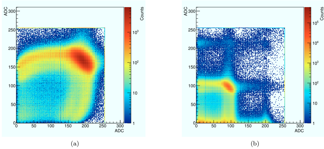
Figure 4: Typical signal of the SYMB in the coincidence mode (a) and Master/Slave mode (b).
