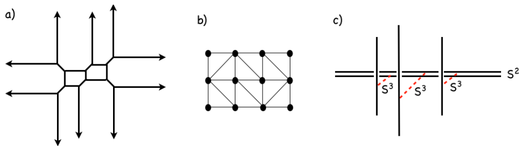
Figure 13. (a) Web diagram of the singularity of interest. (b) Its toric diagram. (c) Complex deformations of the geometry, showing the 3-cycles and the left-over curve of collapsed 2-spheres.
