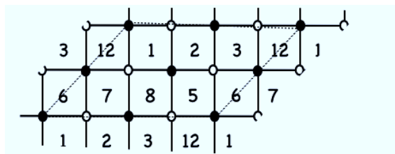
Figure 17. Dimer of the gauge theory at the end of the first cascade.
