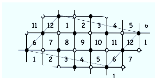
Figure 14. The dimer describing the gauge theory for the underlying system of D3-branes at the singular geometry.
