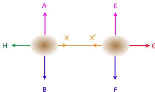
Figure 9. Elongation of the web diagram into two subwebs.
