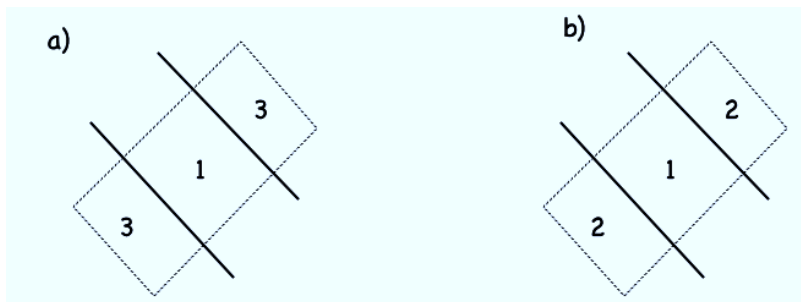
Figure 21. Dimer of the gauge theories after the complex deformation at the bottom of the small throats.
