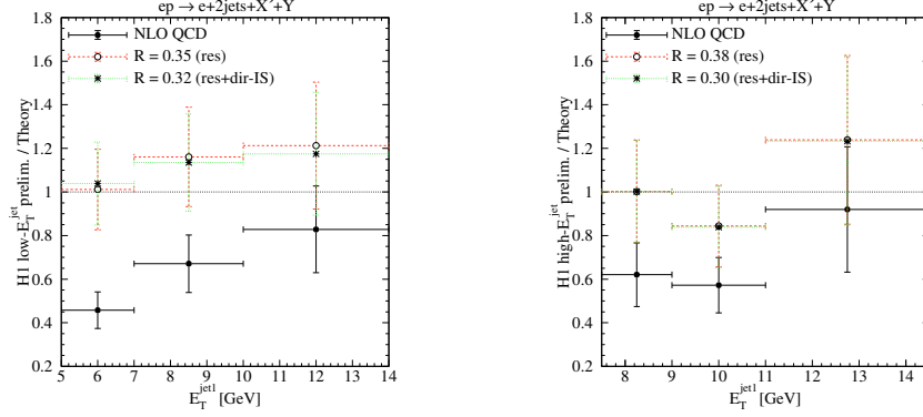
Figure 5. Ratio of the E_T^{jet1} -distribution as measured by H1 with low- E_T^{jet} (left) and high- E_T^{jet} cuts (right) to the NLO QCD prediction without (full), with resolved-only (dashed), and with additional direct IS suppression (dotted) (color online).
