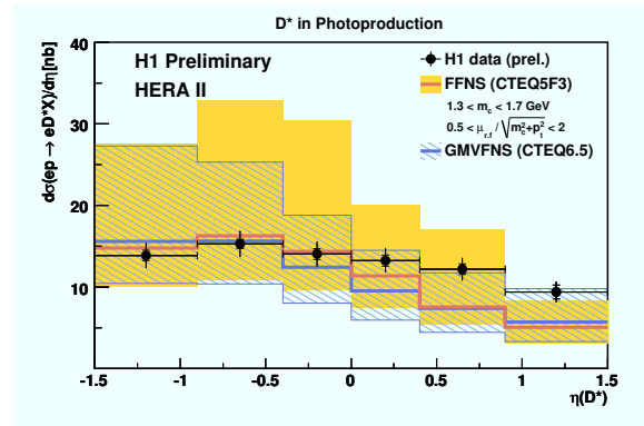
Figure 6. As Fig. 5 for the rapidity distribution d\sigma/d\eta .
