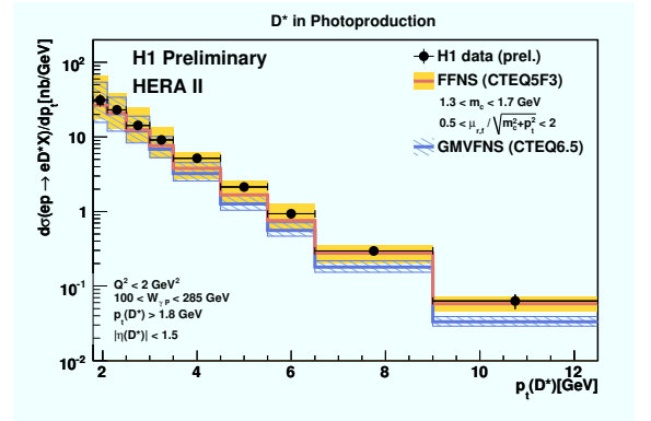
Figure 5. Comparison of NLO predictions in the GM-VFNS for d\sigma/dp_T (hashed (blue) band) with H1 preliminary data [17] for \gamma + p \rightarrow D^* + X . The shaded (yellow) band shows the prediction of a calculation in the fixed-flavor number scheme [3] (see text for further details, colors in the electronic version).
