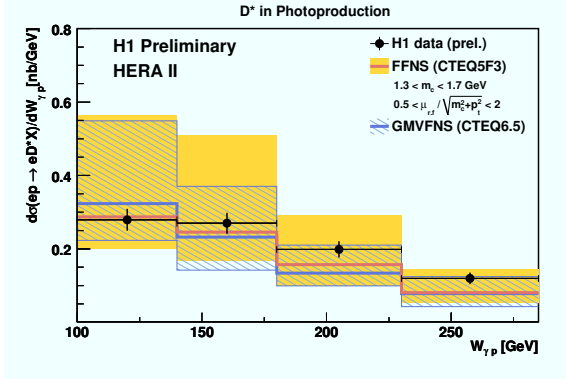
Figure 7. As Fig. 5 for the distribution with respect to the total \gamma p center-of-mass energy, d\sigma/dW_{\gamma p} .
