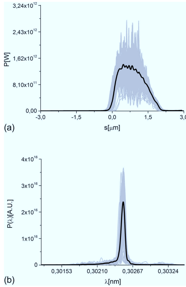
FIG. 5. Power distribution and spectrum of the output radiation pulse for the case of short (4 fs) pulse mode of operation.
