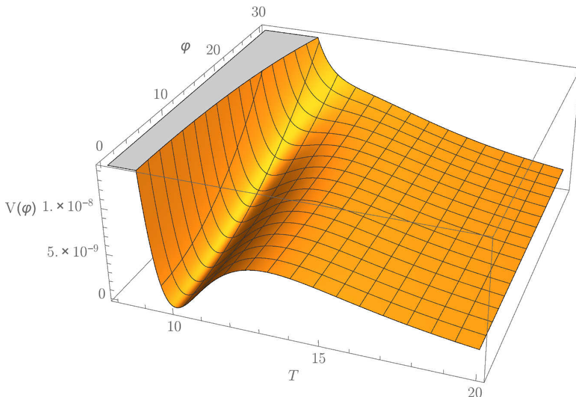
Figure 2. Scalar potential as defined by eqs. (3.17) as a function of T and \varphi , for the same parameter example as in figure 1. Apparently, a minimum for the modulus exists for \varphi \lesssim \varphi_c \approx 24 . Beyond this point the modulus runs away towards T = \infty and can no longer be integrated out. For \varphi < \varphi_c inflation may take place in the valley of the uplifted modulus minimum.
