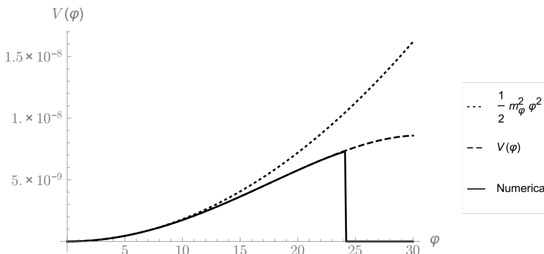
Figure 1. Effective inflaton potential in KKLT for W_0 = 0.009 , A = -0.75 , a = \frac{2\pi}{10} , and m = 1.67 \times 10^{-5} . With these parameters we find T_0 = 10 and m_{3/2} = 10^{-4} . The dotted line denotes a purely quadratic potential with m_\varphi = 6 \times 10^{-6} imposed by COBE normalization. The dashed line is the effective potential eq. (3.27) evaluated at all orders in (aT_0)^{-1} . This potential is valid only as long as the modulus remains stabilized. The solid line is obtained numerically by setting the modulus to its minimum value at each value of \varphi . Evidently, above the critical value \varphi_c \approx 24 the modulus is destabilized towards the run-away minimum at T = \infty and the theory can not be described by eq. (3.27) any longer.
