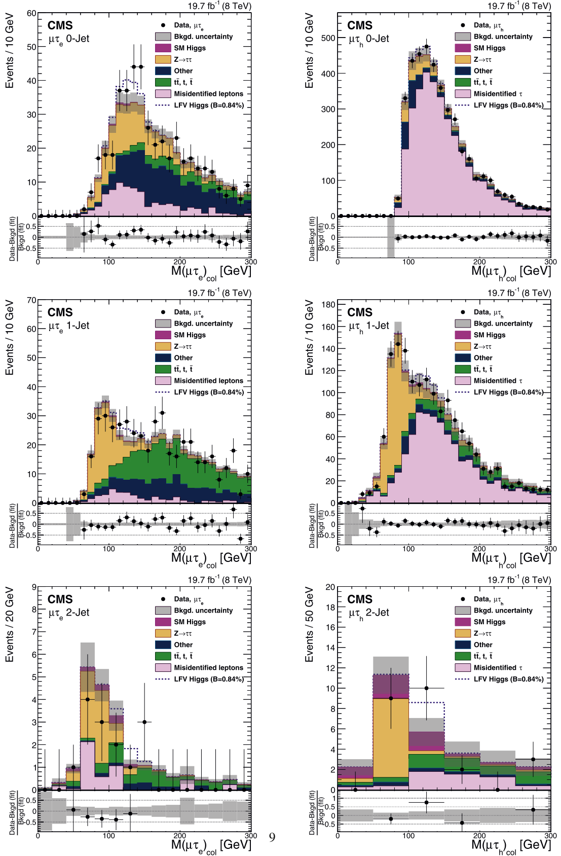
Fig. 3. Distributions of the collinear mass M_{\text{col}} after fitting for signal and background for the LFV H \rightarrow \mu\tau candidates in the different channels and categories compared to data. The distribution of the simulated LFV Higgs boson sample is shown for the best fit branching fraction of \mathcal{B}(H \rightarrow \mu\tau) = 0.84\% . The bottom panel in each plot shows the fractional difference between the observed data and the fitted background. Top left: H \rightarrow \mu\tau_e 0-jet; top right: H \rightarrow \mu\tau_h 0-jet; middle left: H \rightarrow \mu\tau_e 1-jet; middle right: H \rightarrow \mu\tau_h 1-jet; bottom left: H \rightarrow \mu\tau_e 2-jet; bottom right H \rightarrow \mu\tau_h 2-jet.
