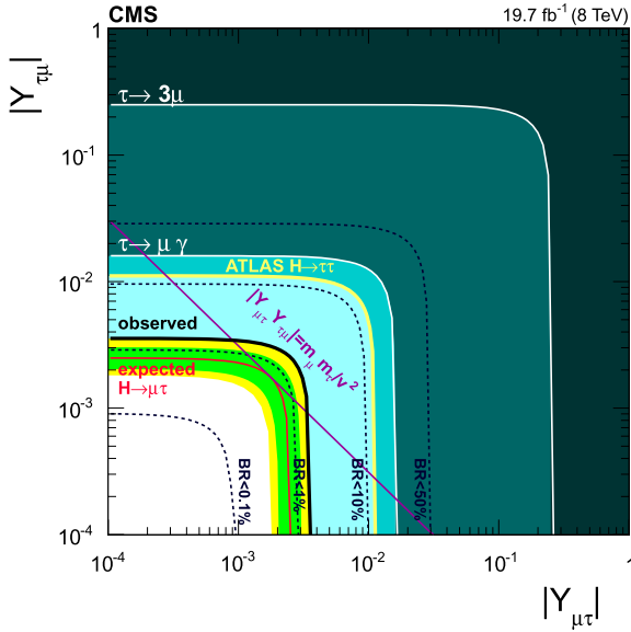
Fig. 6. Constraints on the flavour-violating Yukawa couplings, |Y_{\mu\tau}| and |Y_{\tau\mu}| . The black dashed lines are contours of B(H \rightarrow \mu\tau) for reference. The expected limit (red solid line) with one sigma (green) and two sigma (yellow) bands, and observed limit (black solid line) are derived from the limit on B(H \rightarrow \mu\tau) from the present analysis. The shaded regions are derived constraints from null searches for \tau \rightarrow 3\mu (dark green) and \tau \rightarrow \mu\gamma (lighter green). The yellow line is the limit from a theoretical reinterpretation of an ATLAS H \rightarrow \tau\tau search [4]. The light blue region indicates the additional parameter space excluded by our result. The purple diagonal line is the theoretical naturalness limit Y_{ij}Y_{ji} \leq m_i m_j / v^2 . (For interpretation of the references to color in this figure legend, the reader is referred to the web version of this article.)
