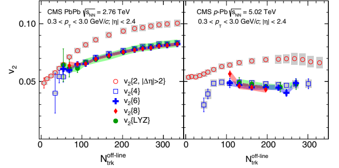
FIG. 2 (color online). The v_2 values as a function of N_{\text{trk}}^{\text{off-line}} . Open data points are the published two- and four-particle v_2 results [35]. Solid data points are v_2 results obtained from six- and eight-particle cumulants, and LYZ methods, averaged over the particle p_T range of 0.3–3.0 GeV/ c , in PbPb at \sqrt{s_{\text{NN}}} = 2.76 TeV (left panel) and p -Pb at \sqrt{s_{\text{NN}}} = 5.02 TeV (right panel). Statistical and systematic uncertainties are indicated by the error bars and the shaded regions, respectively.
