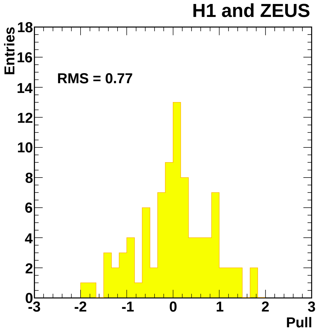
Figure 13: The pull distribution for the combination of the double-differential D^{*\pm} cross sections.
