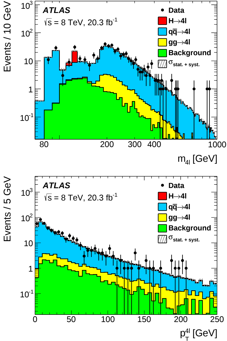
Figure 3: Data and MC prediction comparison for selected events as a function of the invariant mass m_{4\ell} (top) and the transverse momentum p_T^{4\ell} (bottom) of the four-lepton system. The solid colours show the expected contributions from signal and background and the black points represent data with statistical error bars.
