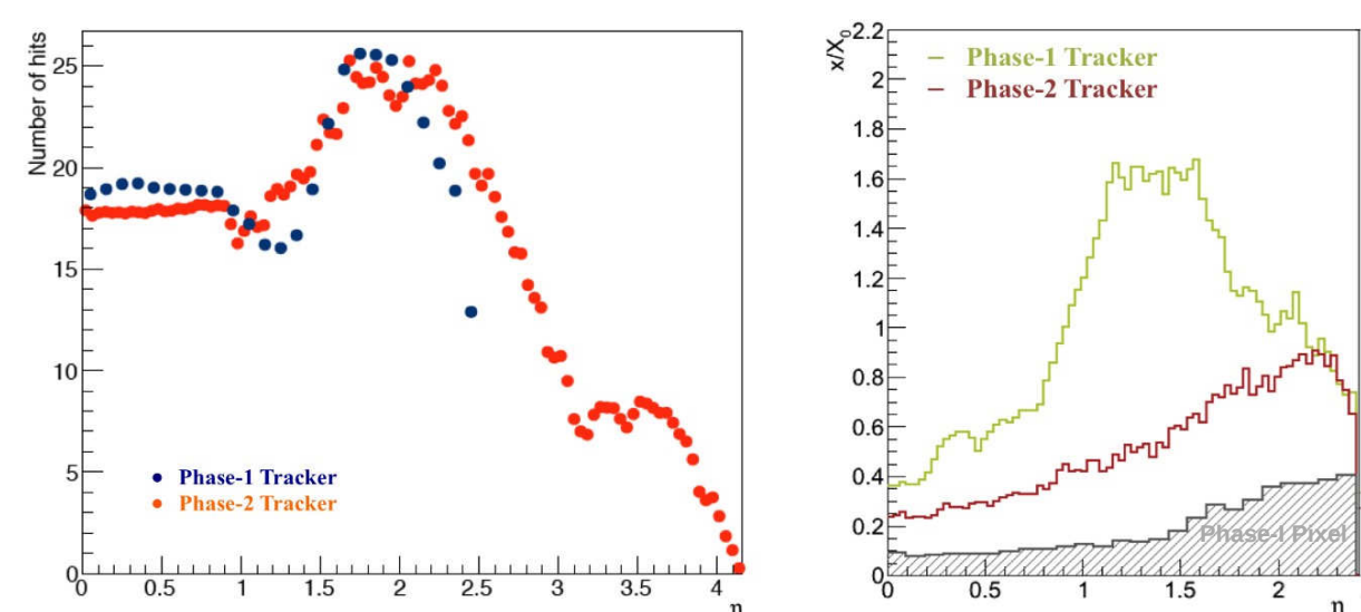
Number of hits (left) and radiation length (right) versus \eta for the Phase-II Tracker and the Phase-I Tracker. The radiation length distribution is shown for the tracking acceptance of the Phase-I Tracker, and reflects only the material inside the tracking volume, the expected contribution of the Phase-I pixel detector (hashed histogram) is provisionally used also for the Phase-II Tracker [1].
