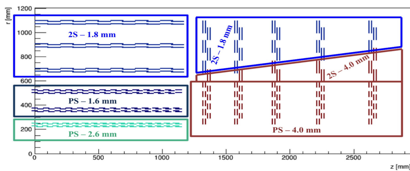
Map of the sensor spacing adopted in the Tracker. The sensor spacing is optimized at the same time as the acceptance window using iLayout, to obtain a P_T threshold of 2 GeV for the stub selection in all module locations. The optimal acceptance window is then recalculated and fine-tuned using the Monte Carlo simulation [1].
