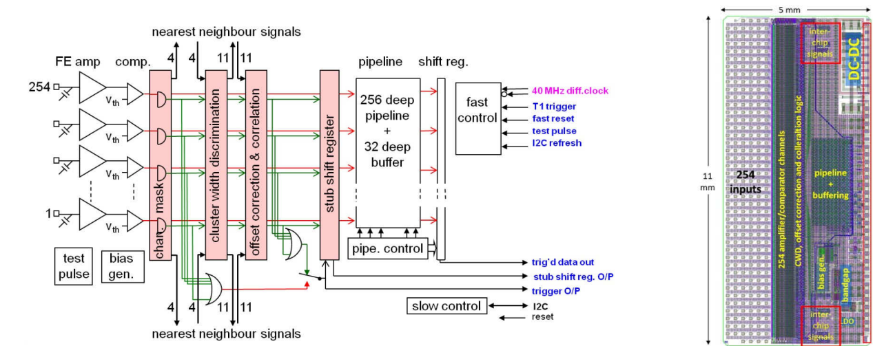
CBC2 block diagram and layout [2].
