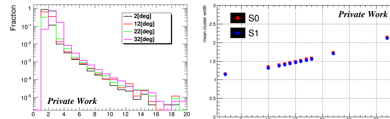
Cluster width distribution vs. rotation. Mean cluster width on DUT sensors (S0 and S1) at different incident angles vs. simulation.
