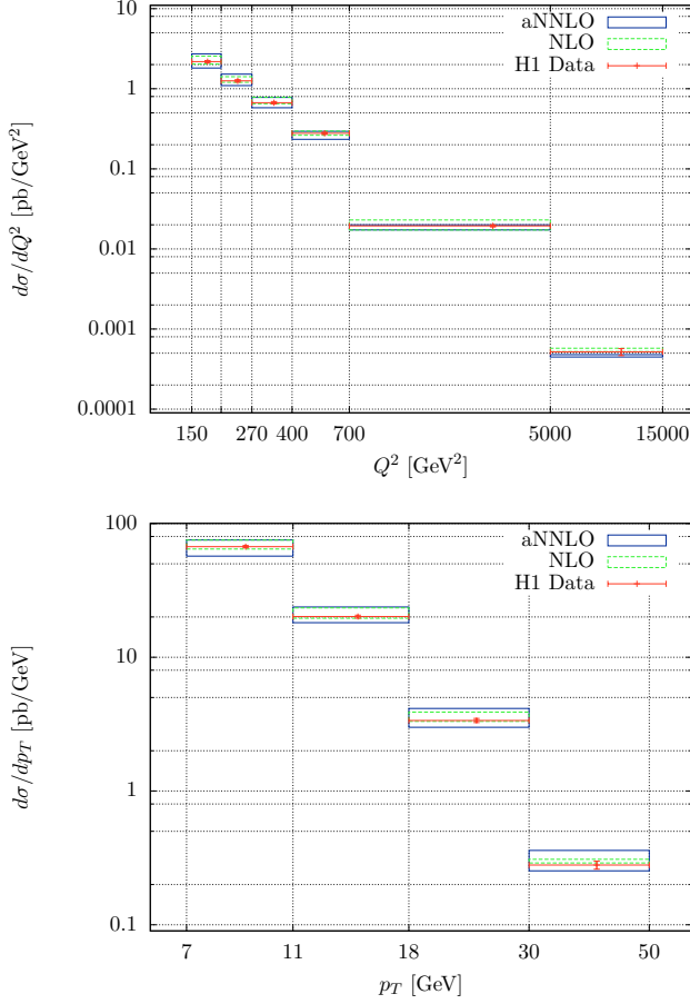
FIG. 1: Single-differential inclusive jet cross sections as a function of photon virtuality Q^2 (top) and jet transverse momentum p_T (bottom) in NLO (green dashed lines) and aNNLO (blue full lines) with the corresponding scale uncertainty bands, obtained by varying \mu_R and \mu_F simultaneously by a factor of two up and down, compared to the final H1 data (red points, color online).
