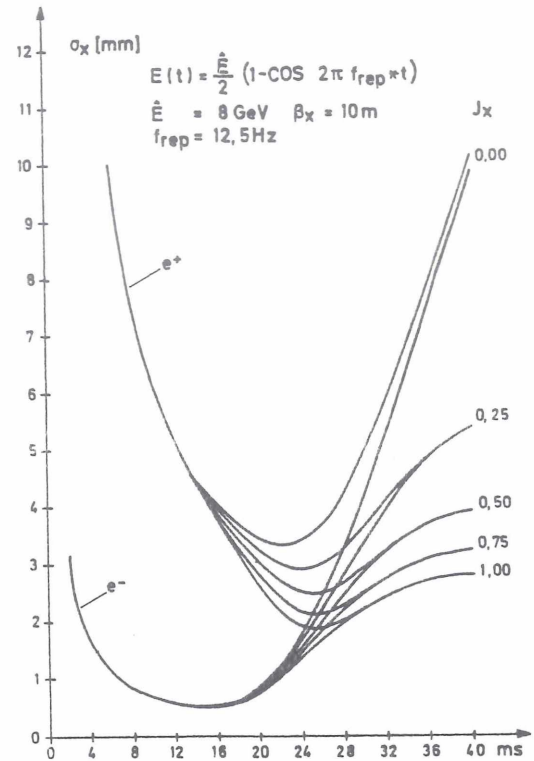
Fig. 4 Horizontal beam size vs. time for 12.5 Hz operation
