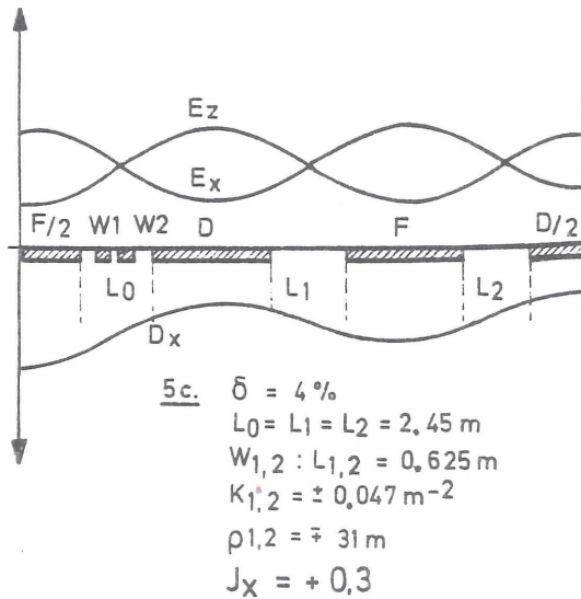
Fig. 5 Various lattice configurations, half cell \Delta p/p = 1\% ; \epsilon_x = \epsilon_z = 40 \pi \text{ mrad mm} ; l_F = l_D = 4.15 \text{ m} B_F/B_D = 1 - \delta ; B_D/B_0 = 1 + \delta
