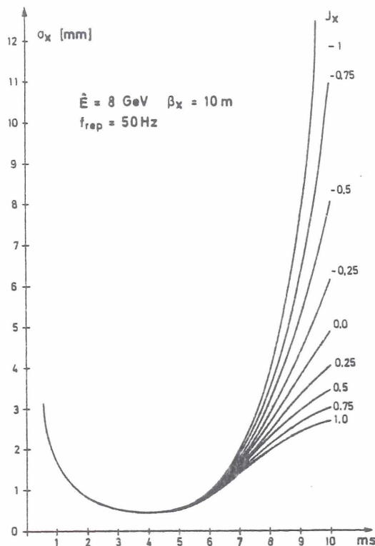
Fig. 3 Horizontal beam size vs. time for 50 Hz cycle frequency
