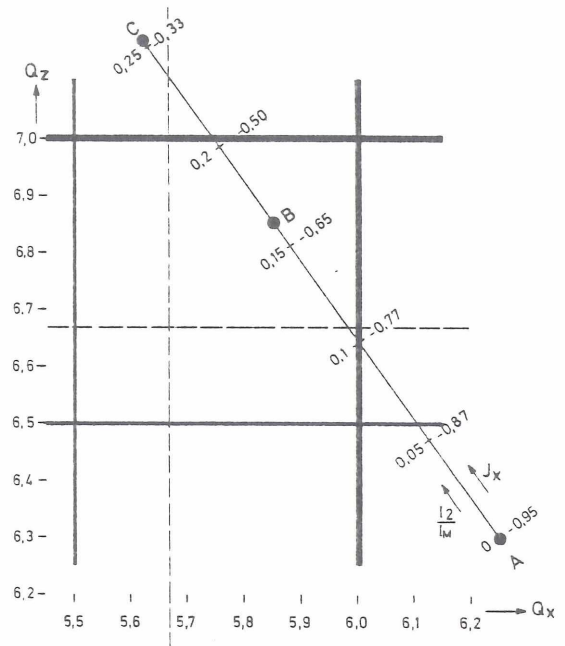
Fig. 7 Working diagram
