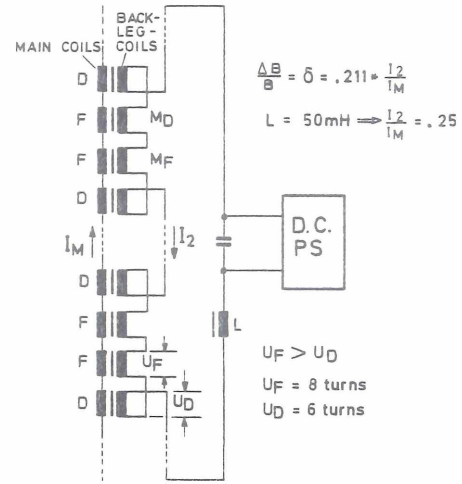
Fig. 6 Backleg circuit
