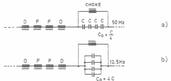
Fig. 2 Magnet circuit a) at present b) proposed
