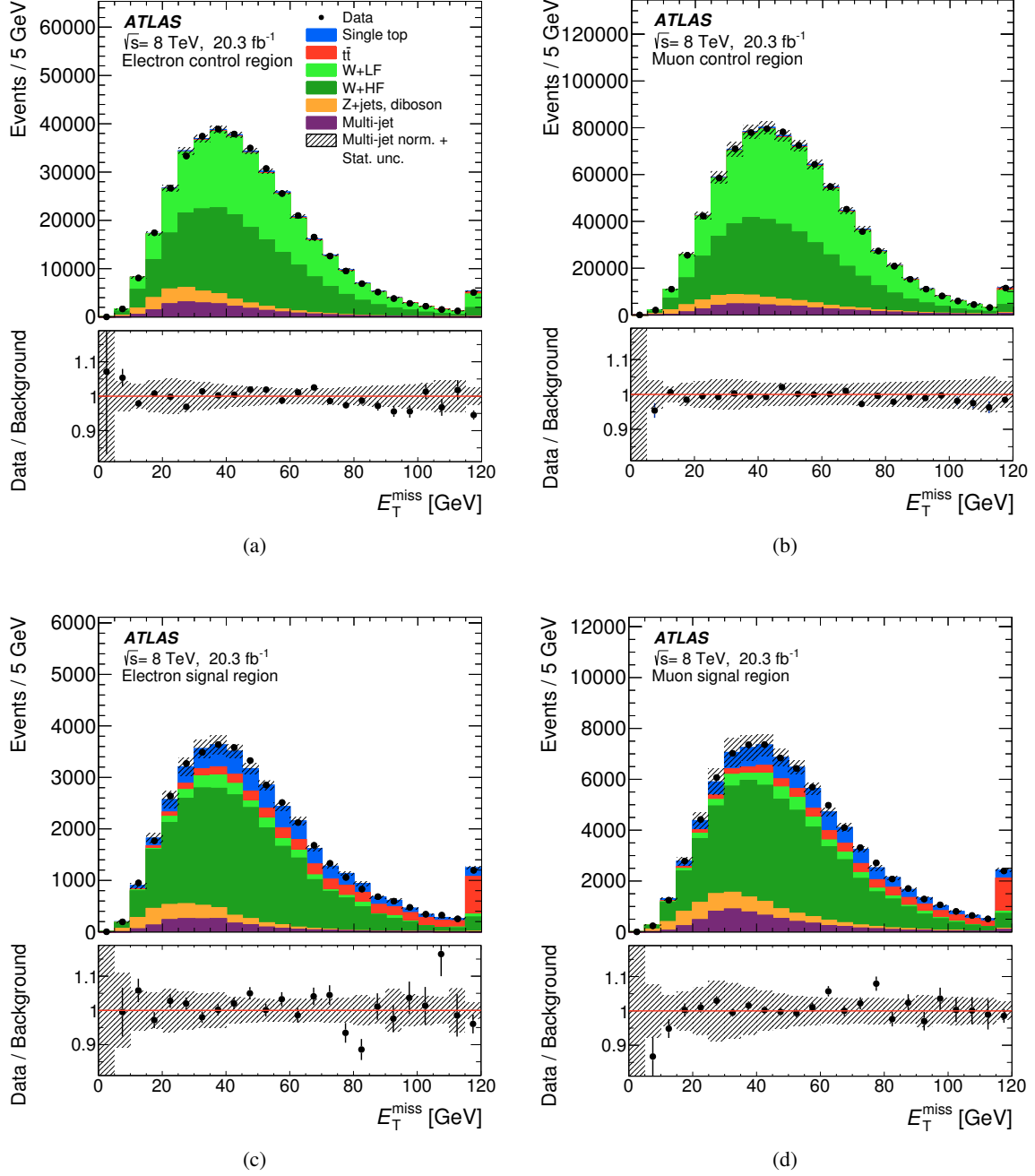
Figure 3: Fitted distributions of the missing transverse momentum E_T^{\text{miss}} for (a) central electrons and (b) muons in the control region and for (c) central electrons and (d) muons in the signal region. The last histogram bin includes overflow events and the hatched error bands contain the MC statistical uncertainty combined with the normalisation uncertainty on the multi-jet background.
