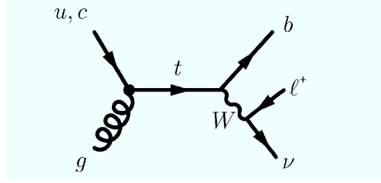
Figure 1: Leading-order Feynman diagram for FCNC top-quark production in the qg \rightarrow t mode followed by the decay of the top quark into a b -quark and a W boson, where the W boson decays into a lepton and a neutrino.
