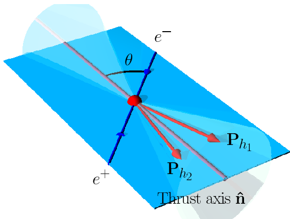
FIG. 2. Illustration of di-hadron fragmentation where the final-state hadrons are depicted as red arrows, the incoming leptons as blue arrows, and the event plane – spanned by leptons and initial quarks/thrust axis – is depicted as a light blue plane. In this case, both hadrons are found in the same hemisphere as defined by the thrust axis, and generally out of the plane, as indicated by the cones.
