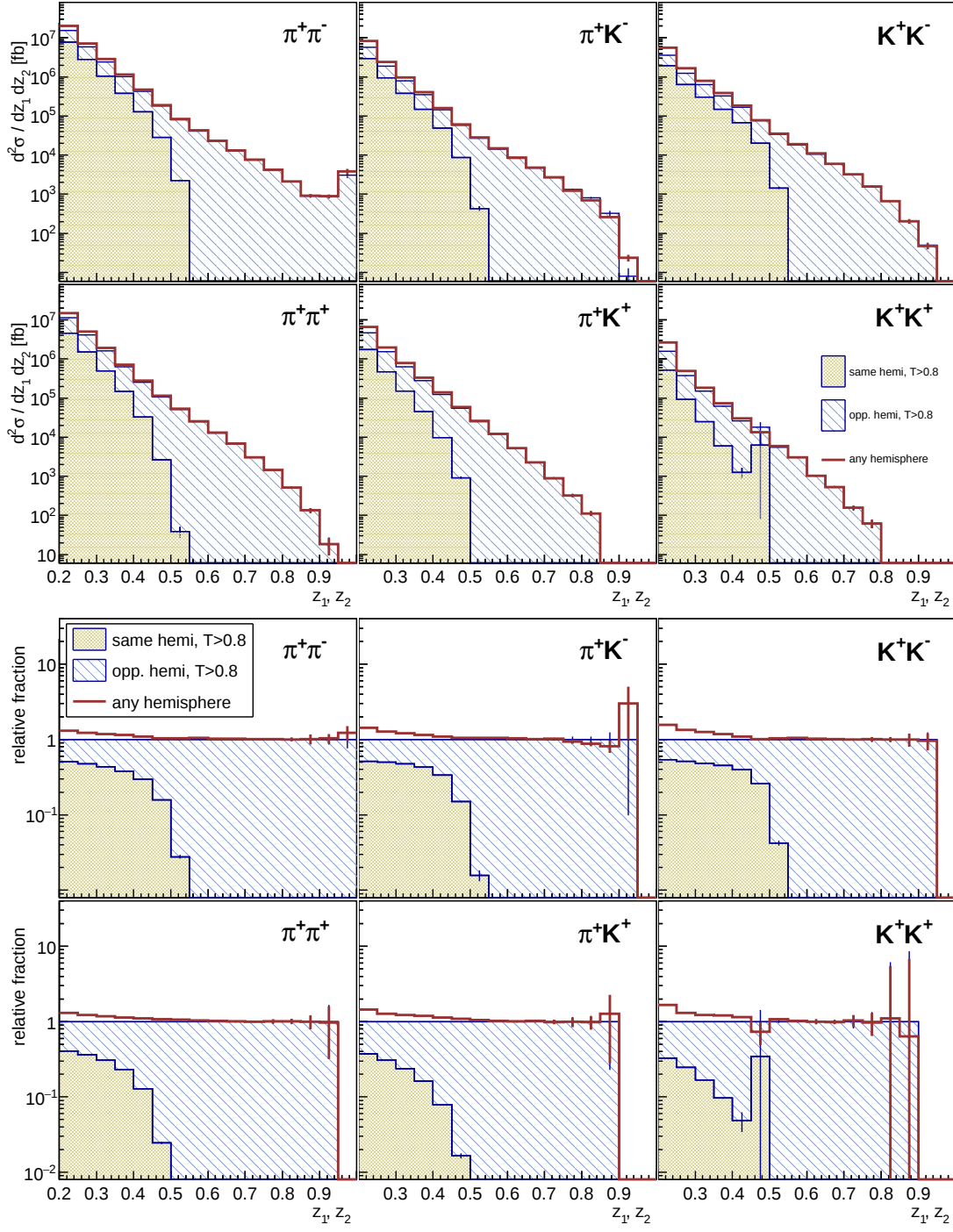
FIG. 17. (color online) Differential cross sections (top) and ratios to the same and opposite topology sum (bottom) for the main hadron combinations stacked between same (gray filled areas, including thrust selection T > 0.8 ) and opposite hemispheres (blue hatched areas, including thrust selection T > 0.8 ) as well as without hemisphere assignment (red curves). For visibility, only the diagonal ( z_1, z_2 ) bins and statistical uncertainties are displayed.
