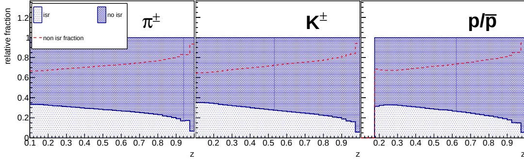
FIG. 21. (color online) Relative fractions for pions, kaons and protons as a function of z_1 originating from ISR or non ISR events. The individual relative contributions are displayed from top to bottom for non ISR events (energy loss less than 0.5%, purple, filled area) and ISR events (blue, hatched area) from generated generic udsc MC. The relative fractions are also shown for the non-ISR fraction (green, dashed lines).
