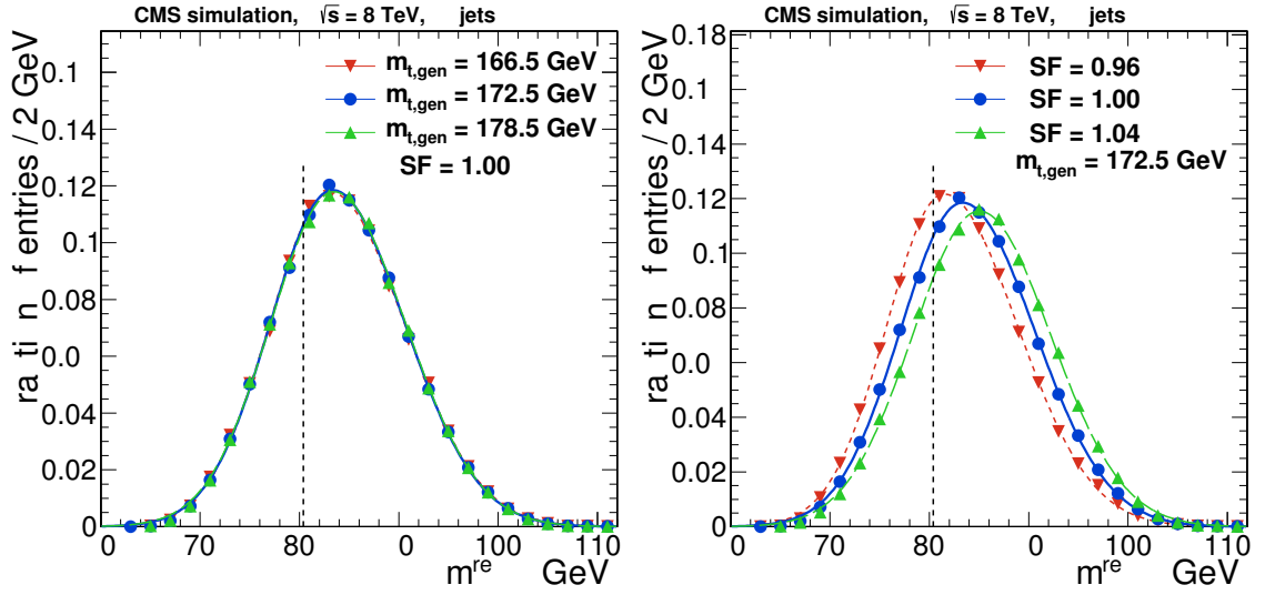
Figure 7.7.: Simulated m_W^{\text{reco}} distributions of correct t\bar{t} permutations, for three generated masses m_{t,\text{gen}} with JSF = 1 (left), and for three jet scale factors with m_{t,\text{gen}} = 172.5 GeV (right). The vertical dashed line indicates the known W -boson mass of m_W = 80.4 GeV.
