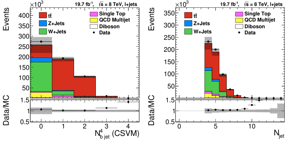
Figure 6.2.: Preselection: Number of b-tagged jets among the four leading jets with p_T > 30 \text{ GeV} , (left), and number of jets with p_T > 20 \text{ GeV} .
