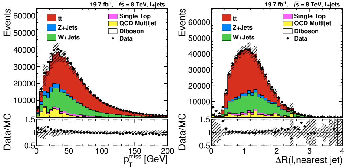
Figure 6.3.: Preselection: Missing transverse momentum (left), and minimum distance between the selected lepton and a jet with p_T > 20 \text{ GeV} (right).
