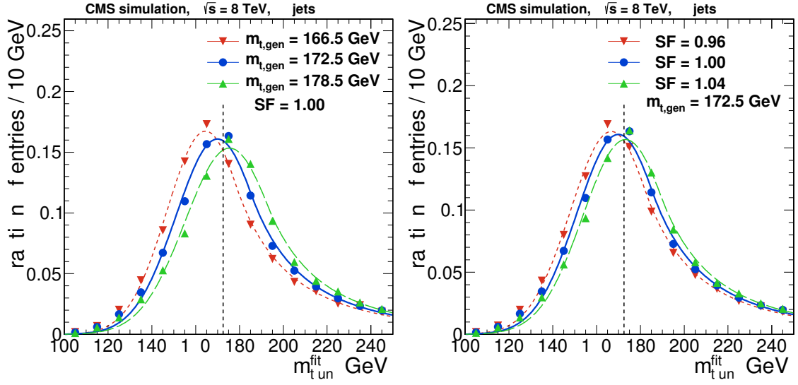
Figure 7.6.: Simulated m_t^{\text{fit}} distributions of unmatched t\bar{t} permutations, for three generated masses m_{t,\text{gen}} with JSF = 1 (left), and for three jet scale factors with m_{t,\text{gen}} = 172.5 GeV (right). The vertical dashed line corresponds to m_t^{\text{fit}} = 172.5 GeV.
