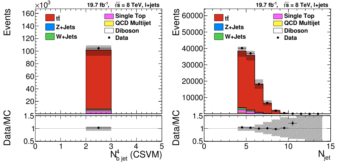
Figure 6.5.: Baseline selection: Number of b-tags among the four leading jets with p_T > 30 GeV, (left), and number of jets with p_T > 20 GeV.
