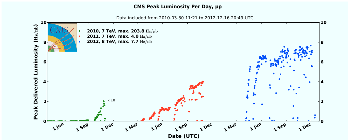
Figure 4.2.: Peak luminosity delivered to CMS in proton-proton collisions. Source: CMS collaboration [99].
