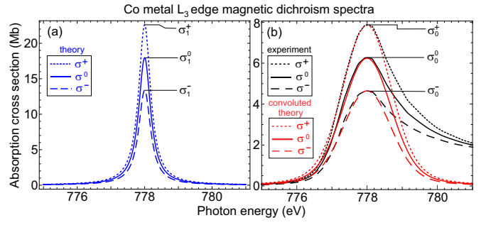
FIG. 1: (a) Polarization and photon energy dependent L_3 absorption cross sections \sigma_{\text{abs}}^q = 2\lambda f''^q for Co metal, calculated by use of Eq. 2 and the parameters \Gamma and \Gamma_x^q in Table I. (b) Comparison of the experimental dichroic cross sections (black lines) and the theoretical cross sections in (a) convoluted with a Gaussian of 1.4 eV FWHM. Note that the corresponding blue and red curves have the same areas but their peak values differ by a factor of \sigma_1^q/\sigma_0^q = 2.9 .
