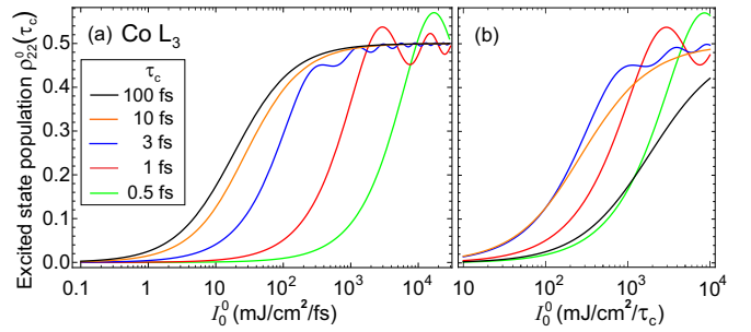
FIG. 2: (a) \tilde{\rho}_{22}^q(\tau_c) as a function of linearly polarized incident intensity I_0^0 for different coherence times \tau_c of the incident pulses for the L_3 edge of a 20 nm thick Co metal film. We assumed resonance excitation, \hbar\omega = \mathcal{E}_0 , and experimental peak cross sections as discussed in the text. (b) Same as in (a) as a function of the incident fluence per coherence time of the pulse.
