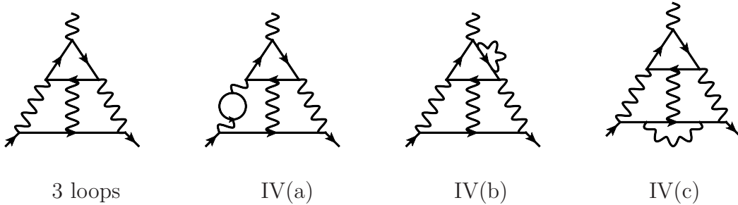
Figure 1: Sample light-by-light-type Feynman diagrams contributing to a_\mu . The external solid line represents the muon and at least one of the internal solid loops denotes electrons. In the case of IV(a) the second fermion loop can either be an electron or muon loop. Wavy lines represent photons.
