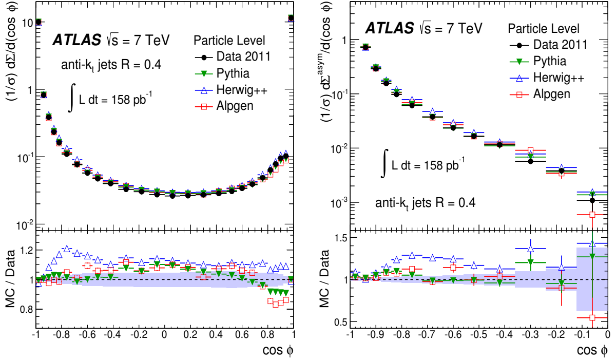
Figure 3: The unfolded distributions for transverse energy–energy correlation (left) and its asymmetry (right) along with comparisons to MC expectations. The statistical uncertainties are shown with error bars, while the total experimental uncertainties are shown in a shaded band.
