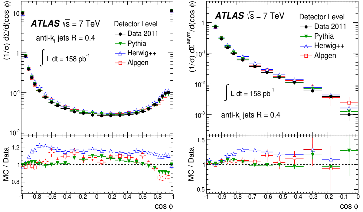
Figure 1: The detector-level distributions for the transverse energy–energy correlation TEEC (left) and its asymmetry ATEEC (right) along with comparisons to MC model expectations. The uncertainties shown are statistical only. The first bin of the ATEEC distribution has a negative value and is therefore not included in the figure.
