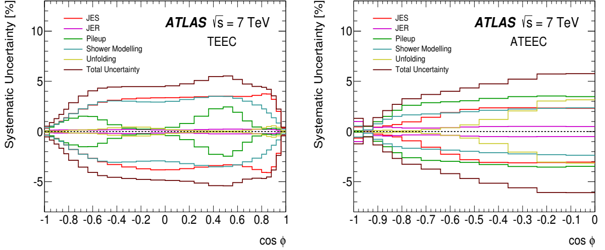
Figure 2: Relative systematic uncertainties for the TEEC (left) and the ATEEC (right) as a function of \cos \phi .
