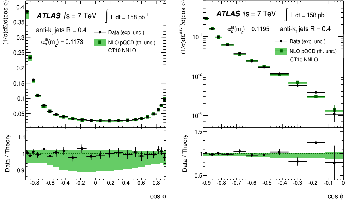
Figure 4: The unfolded distributions for transverse energy–energy correlation (left) and its asymmetry (right) compared with the results of a fit to pQCD NLO calculations including non-perturbative corrections. The green shaded band indicates the uncertainty on the theoretical predictions, which includes the sum in quadrature of uncertainties associated with scale, \alpha_s , PDF and NPC. The statistical uncertainties on the predictions are indicated by green error bars, appreciable only on the tail of the ATEEC. The solid error bars on the data points (in black) indicate the experimental uncertainties taking into account the correlations between them. The fitted values of the strong coupling constant are \alpha_s^{\text{fit}}(m_Z) = 0.1173 (TEEC) and \alpha_s^{\text{fit}}(m_Z) = 0.1195 (ATEEC).
