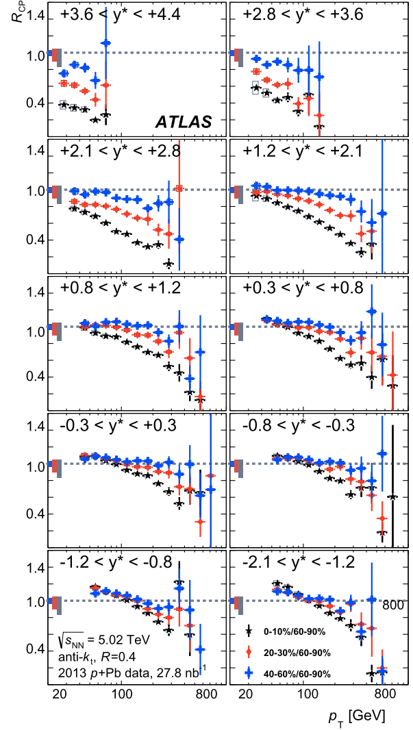
Fig. 4. Measured R_{CP} values for R = 0.4 jets in p + \text{Pb} collisions in central (stars), mid-central (diamonds) and mid-peripheral (crosses) events. Each panel shows the jet R_{CP} in a different rapidity range. Vertical error bars represent the statistical uncertainty while the boxes represent the systematic uncertainties on the jet yields. The shaded boxes at the left edge of the R_{CP} = 1 horizontal line indicate the systematic uncertainty on R_{coll} for (from left to right) peripheral, mid-central and central events.
