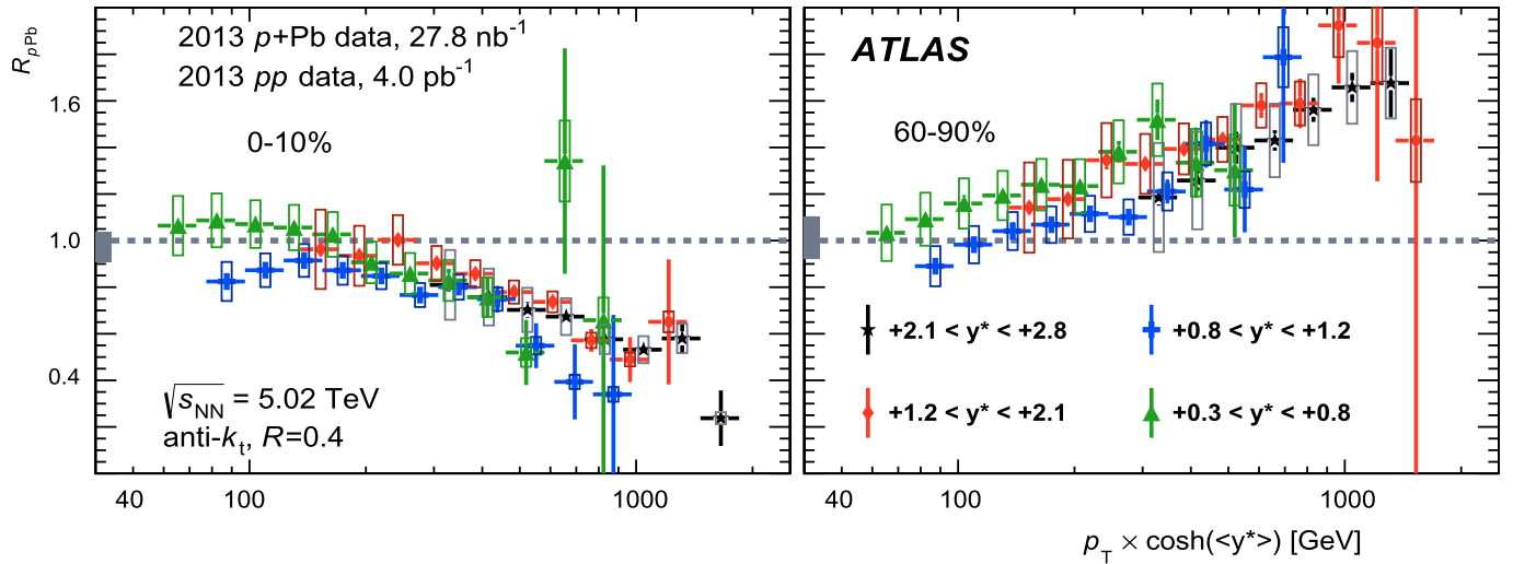
Fig. 7. Measured R_{pPb} values for R = 0.4 jets in p + \text{Pb} collisions displayed for multiple rapidity ranges, showing 0–10% events in the left panel and 60–90% events in the right panel. The R_{pPb} at each rapidity is plotted as a function of p_T \times \cosh(\langle y^* \rangle) , where \langle y^* \rangle is the midpoint of the rapidity bin. Vertical error bars represent the statistical uncertainty while the boxes represent the systematic uncertainties on the jet yields. The shaded box at the left edge of the R_{pPb} = 1 horizontal line indicates the systematic uncertainties on T_{pA} and the pp luminosity added in quadrature.
