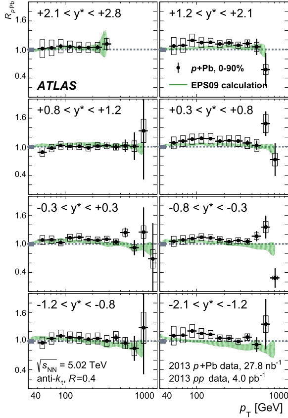
Fig. 3. Measured R_{pPb} values for R = 0.4 jets in 0–90% p + \text{Pb} collisions. Each panel shows the jet R_{pPb} in a different rapidity range. Vertical error bars represent the statistical uncertainty while the boxes represent the systematic uncertainties on the jet yields. The shaded box at the left edge of the R_{pPb} = 1 horizontal line indicates the systematic uncertainty on T_{pA} and the pp luminosity in quadrature. The shaded band represents a calculation using the EPS09 nuclear parton distribution function set.
