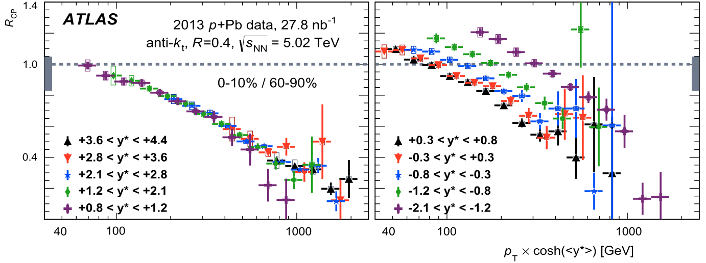
Fig. 6. Measured R_{CP} values for R = 0.4 jets in 0–10% p + \text{Pb} collisions. The panel on the left shows the five rapidity ranges that are the most forward-going, while the panel on the right shows the remaining five. The R_{CP} values at each rapidity are plotted as a function of p_T \times \cosh(\langle y^* \rangle) , where \langle y^* \rangle is the midpoint of the rapidity bin. Vertical error bars represent the statistical uncertainty while the boxes represent the systematic uncertainties on the jet yields. The shaded box at the left edge (in the left panel) and right edge (in the right panel) of the R_{CP} = 1 horizontal line indicates the systematic uncertainty on R_{coll} .
