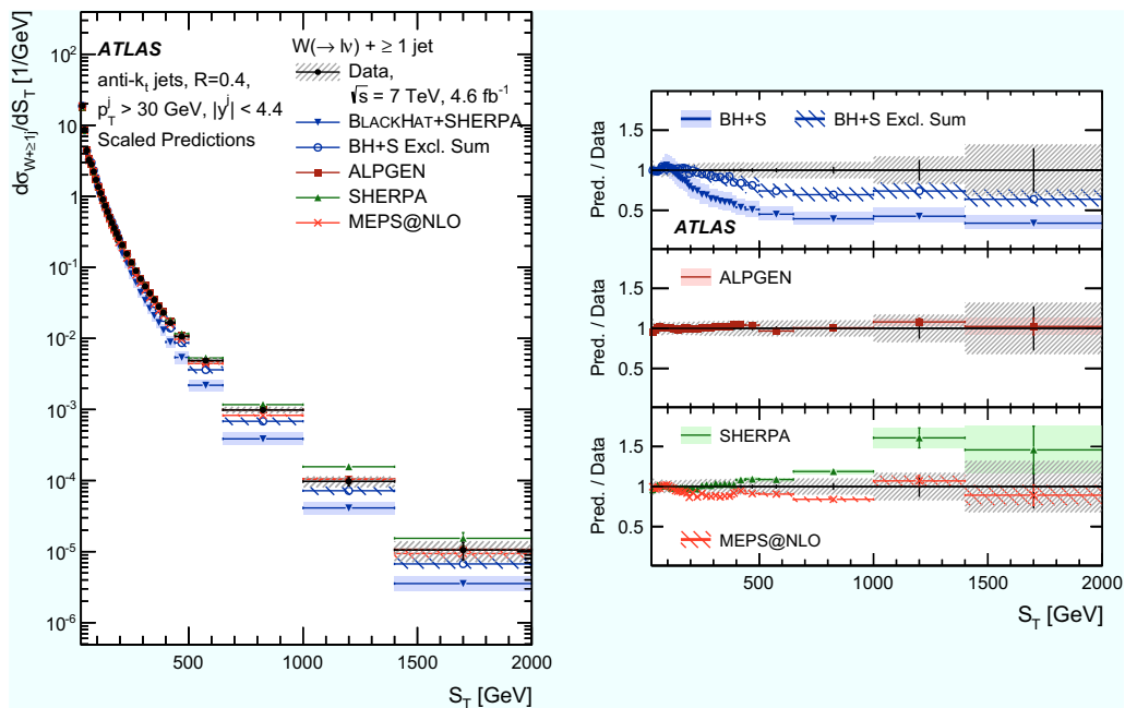
Fig. 32 Cross section for the production of W + \text{jets} as a function of the S_T in N_{\text{jet}} \geq 1 events. For the data, the statistical uncertainties are shown by the vertical bars , and the combined statistical and systematic uncertainties are shown by the black-hashed regions . The data are compared to predictions from BLACKHAT+SHERPA, BLACKHAT+SHERPA including the exclusive summing, ALPGEN, SHERPA
