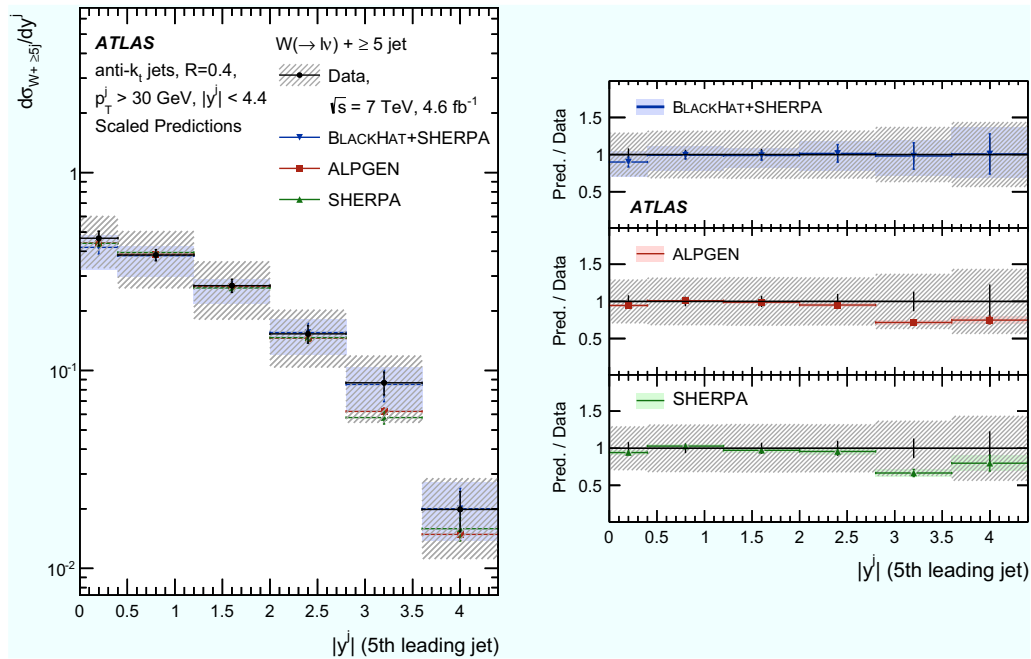
Fig. 31 Cross section for the production of W + \text{jets} as a function of the fifth leading jet rapidity in N_{\text{jets}} \geq 5 events. For the data, the statistical uncertainties are shown by the vertical bars , and the combined statistical and systematic uncertainties are shown by the black-hashed regions . The data are compared to predictions from BLACKHAT+SHERPA, ALPGEN, and SHERPA. The left-hand plot shows the
