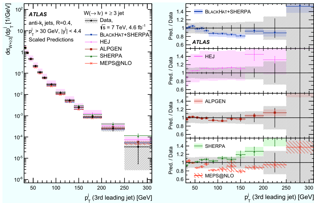
Fig. 12 Cross section for the production of W + \text{jets} as a function of the third leading-jet p_T in N_{\text{jets}} \geq 3 events. For the data, the statistical uncertainties are shown by the vertical bars, and the combined statistical and systematic uncertainties are shown by the black-hashed regions. The data are compared to predictions from BLACKHAT+SHERPA, HEJ, ALPGEN, SHERPA and MEPS@NLO. The left-hand plot shows the
