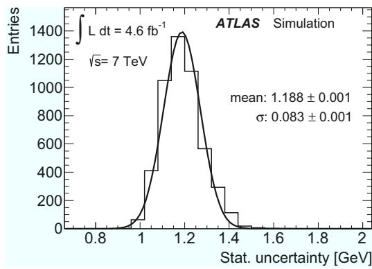
Fig. 6 Expected statistical uncertainty on the top-quark mass obtained from 5000 pseudo-experiments using t\bar{t} MC simulation events assuming m_t = 175 GeV and neglecting correlations between the two R_{3/2} values per event
