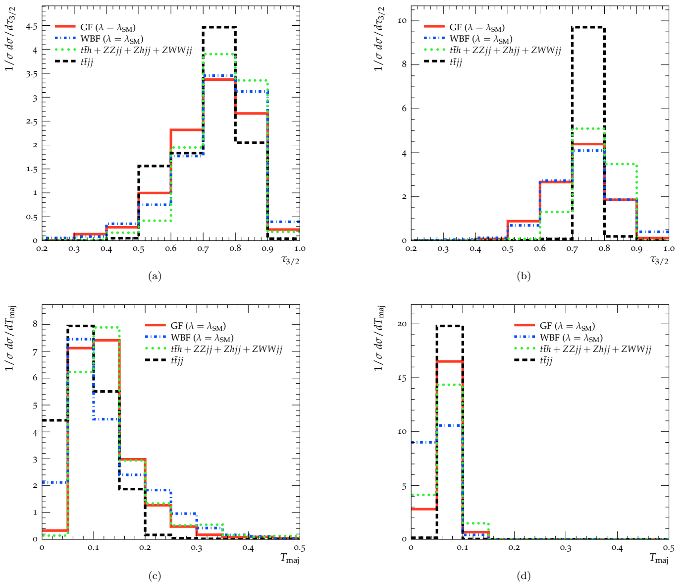
FIG. 9: Shape comparisons of N -jettiness and thrust calculated in the major direction after the gluon fusion selection of Sec. IV A (a,c) and WBF Selection of Sec. IV B (b,d) have been applied.
