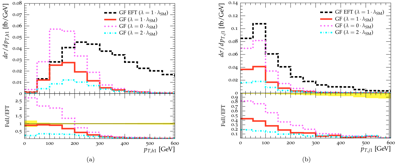
FIG. 1: Maximum Higgs and jet transverse momenta for gluon fusion-induced hhjj production, including the ratio of full theory to the effective theory calculation for three different values of the Higgs trilinear coupling \lambda .
