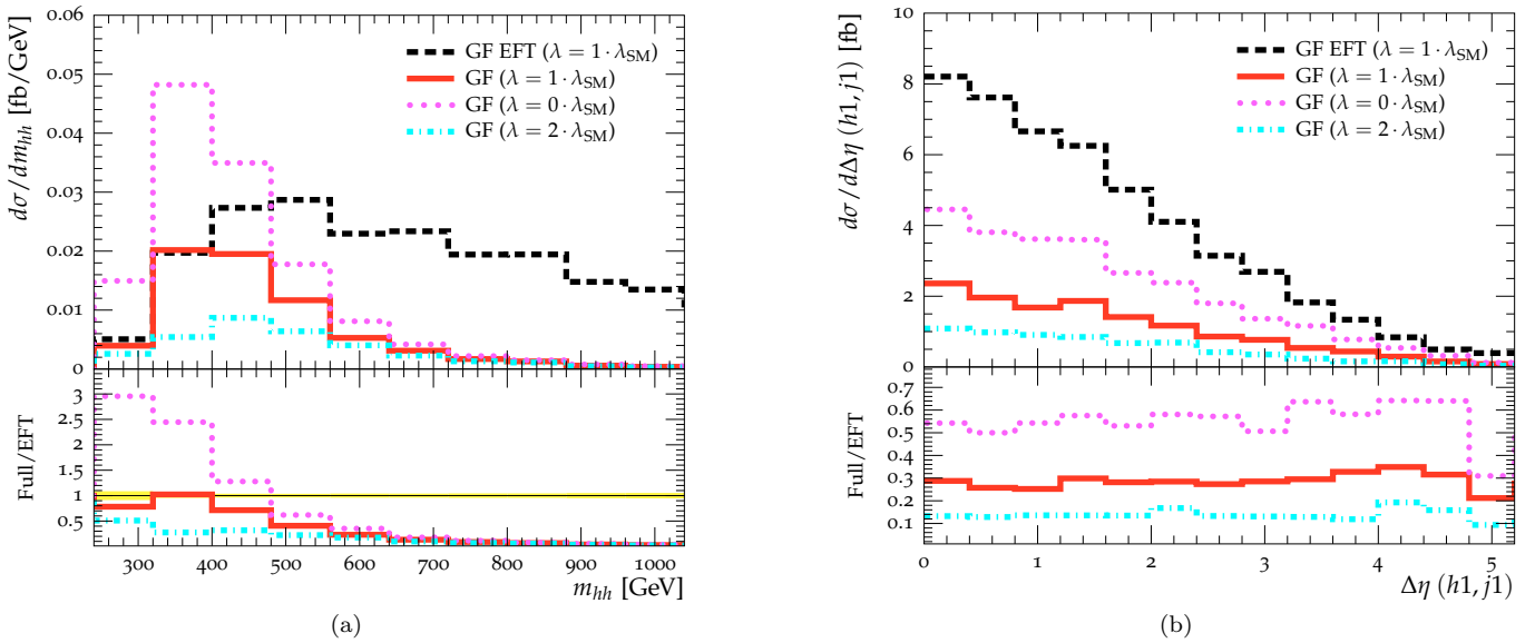
FIG. 4: Invariant mass and pseudo-rapidity distributions of the leading jet and di-Higgs system in QCD-mediated hhjj production. We show the effective theory and full theory results for three values of the trilinear Higgs coupling, applying only generator-level cuts of p_{T,j} \geq 20 GeV and |\eta_j| < 5 .
