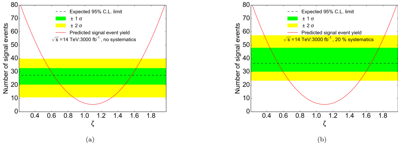
FIG. 8: Expected limits on the gauge-Higgs quartic couplings \zeta = g_{VVhh}/g_{VVhh}^{\text{SM}} under the assumption of no systematic uncertainties (a) and 20% systematic uncertainties (b).
