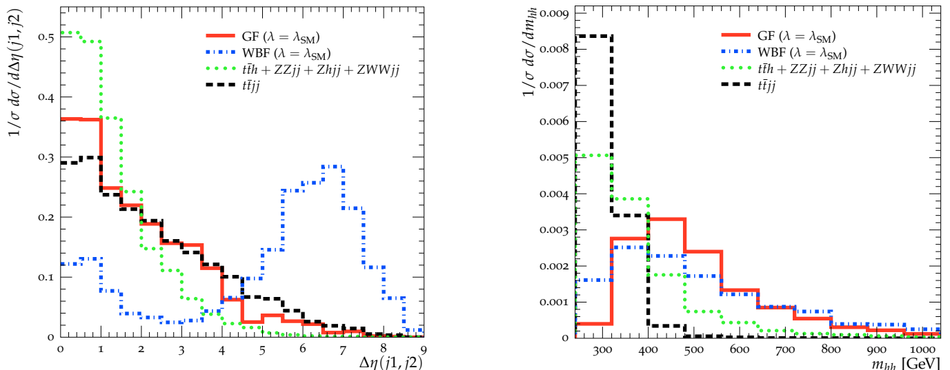
FIG. 7: Shape comparison of \Delta\eta(j1, j2) and m_{hh} distributions for our two sources of signal (GF and WBF), the dominant background t\bar{t}jj and the rest of the backgrounds (stacked scaled by relative cross sections), after the Base Selection of Section IV has been applied.
