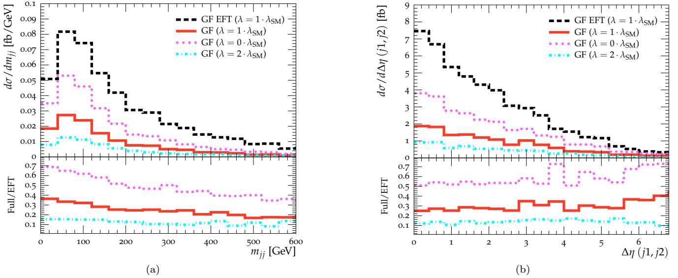
FIG. 3: Invariant mass and pseudo-rapidity distributions of the jet system in QCD-mediated hhjj production. We show the effective theory and full theory results for three values of the trilinear Higgs coupling, applying only generator-level cuts of p_{T,j} \geq 20 GeV and |\eta_j| < 5 .
