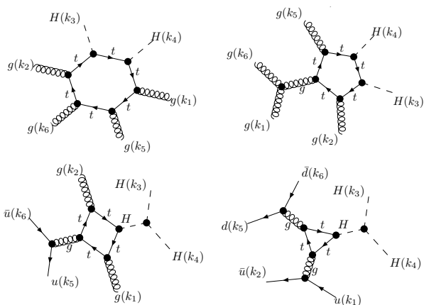
FIG. 2: Sample Feynman diagrams contributing to pp \rightarrow hhjj via gluon fusion.
